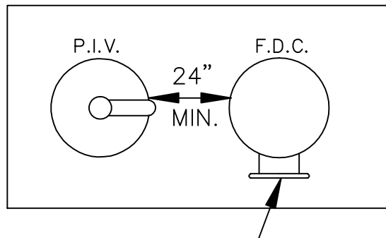
5" STORZ CONNECTION @ 30 DEG. ANGLE WITH CAP
